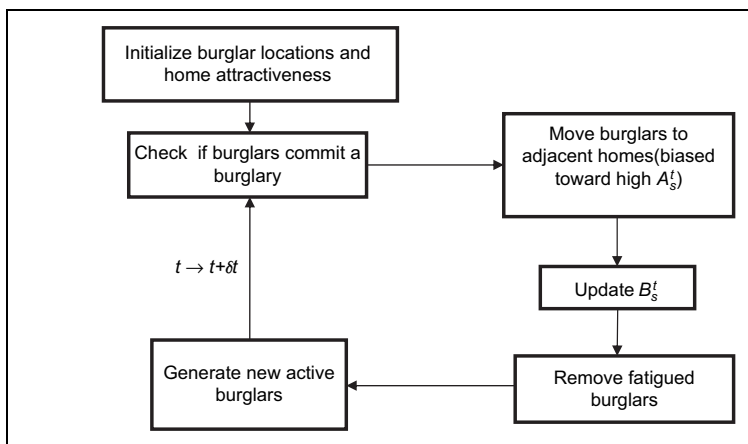
Figure 2. Overview of the algorithm used in the simulation.
