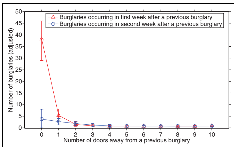
Figure 6. Results of 25 simulations for the boost model with homogeneous risks across homes (error bars show minimum and maximum values).
