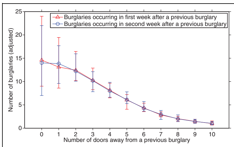
Figure 3. Results of 25 simulations for the model with heterogeneous risks across homes (spots configuration; error bars show minimum and maximum values).
