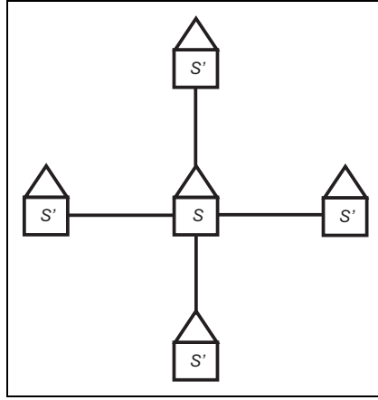
Figure 1. Four nearest neighbors on the square lattice (Von Neumann neighborhood).
