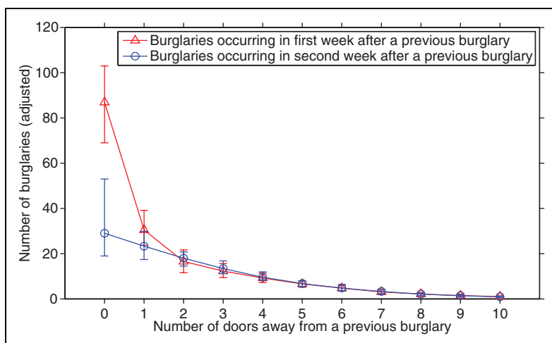
Figure 7. Results of 25 simulations for the boost model with heterogeneous risks across homes (spots configuration; error bars show minimum and maximum values).
