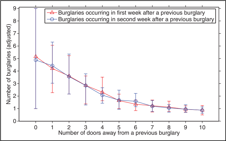
Figure 4. Results of 25 simulations for the model with heterogeneous risks across homes (stripe configuration; error bars show minimum and maximum values).
